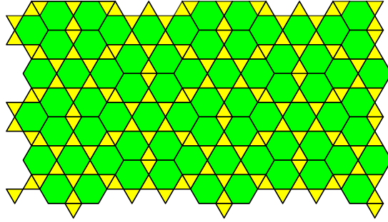
FIGURE 4. A tiling with isolated 3-valent vertices. Figure modified from [33].
