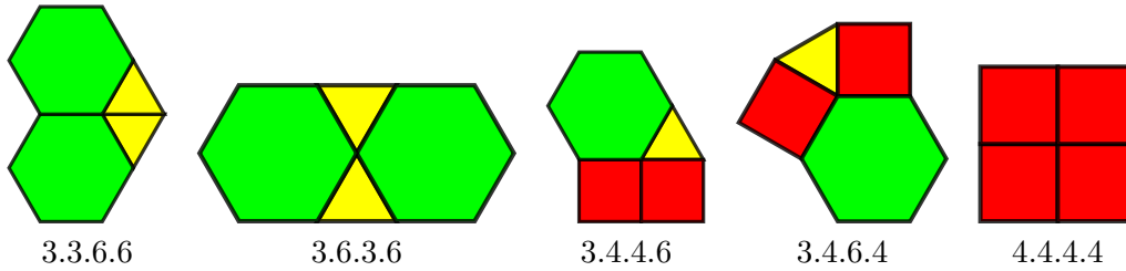
FIGURE 5. Allowable vertex types for tilings with only 4-valent vertices.
