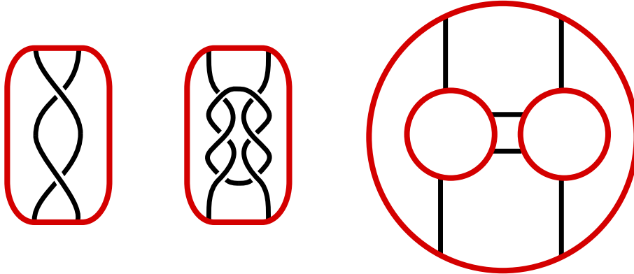
FIGURE 2.8. Three tangles represented by two-dimensional projections. The first one is trivial in a three-ball, the second one is non-trivial in a three-ball and the third one is flat in the solid pants.
