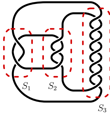
FIGURE 3.3. The pretzel knot P(-2, 3, 7) with a sphere-decomposition made of three spheres S_1 , S_2 and S_3 1 .
