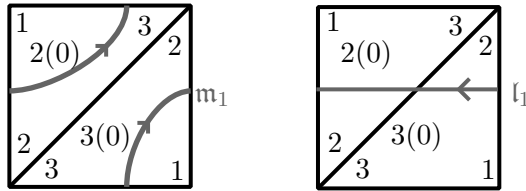
FIGURE 9. Choices for \mathbf{m}_1 and \mathbf{l}_1 .
