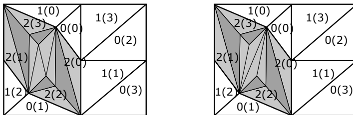
FIGURE 8. Cusp triangulations of manifolds obtained by 1/2 and -1/1 Dehn fillings. The shaded triangles come from the layered solid torus.
