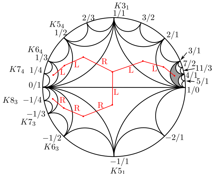
FIGURE 7. Paths in the Farey triangulation that produce knots obtained by Dehn filling the Whitehead sister.
