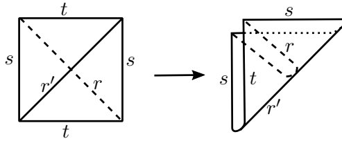
FIGURE 6. Folding makes the diagonal slope r homotopically trivial.
