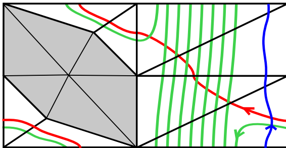
FIGURE 4. The preferred longitude \ell' = \text{Im}^{-8} is shown in green.
