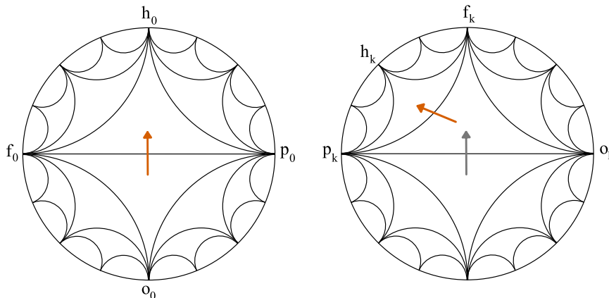
FIGURE 11. Slope labels for the k th step. Left: k = 0 . Right: k > 0 .
