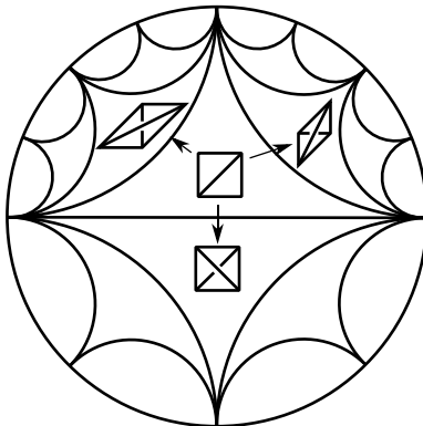
FIGURE 5. Tetrahedra obtained from moving across triangles in the Farey triangulation.
