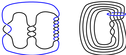
FIGURE 1. Two views of the (-2, 3, 8) -pretzel link. One component (shown in blue) is an unknot embedded in S^3 .
