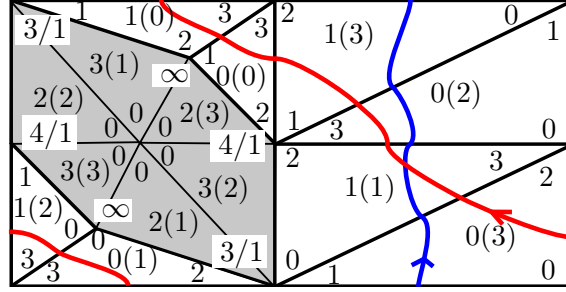
FIGURE 3. Triangulation of the unfilled cusp of the Whitehead sister. Generators of homology are shown: \mathfrak{l} in red and \mathfrak{m} in blue.
