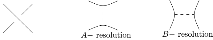
FIGURE 3. A - and B -resolutions of a crossing.
