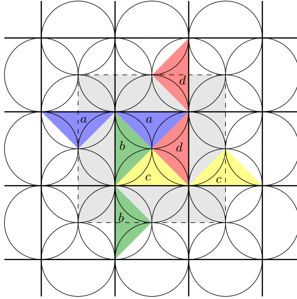
FIGURE 7. Face pairings for a fundamental domain \mathcal{P}_W of \mathbb{R}^3 - \mathcal{W} . The shaded part indicates the fundamental domain of S^3 - L .
