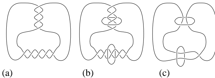
FIGURE 2. (a) The original link diagram K . (b) Crossing circles added. (c) The diagram of L .
