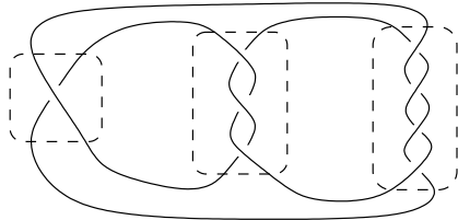
FIGURE 1. Twist regions of the diagram are encircled with dashed lines. For this diagram, tw(D_K) = 3 .
