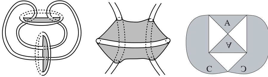
FIGURE 3. Decomposing S^3 - L into ideal polyhedra: First slice along the projection plane, then split remaining halves of two-punctured disks. Obtain polyhedron on right.
