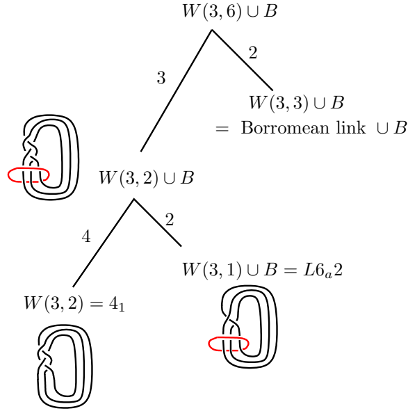
FIGURE 7. The complement of the figure-8 knot and its braid axis, S^3 - (W(3,2) \cup B) , is a 4-fold cover of the figure-8 knot complement, S^3 - W(3,2) .
