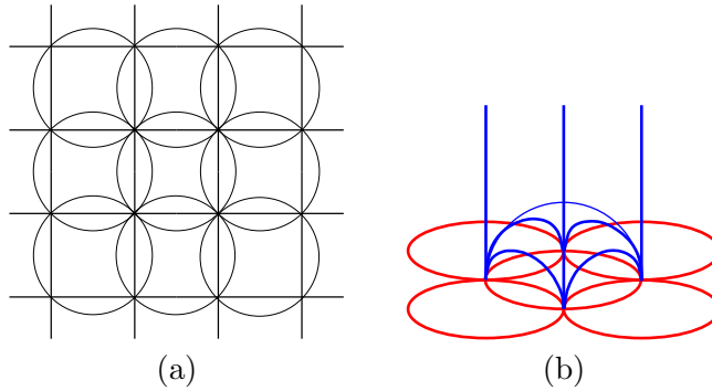
FIGURE 10. (a) Circle pattern for hyperbolic planes of the top polyhedron of \mathbb{R}^3 - \mathcal{W} . (b) Hyperbolic planes bounding one top square pyramid.
