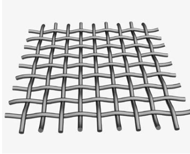
FIGURE 2. The infinite alternating weave
