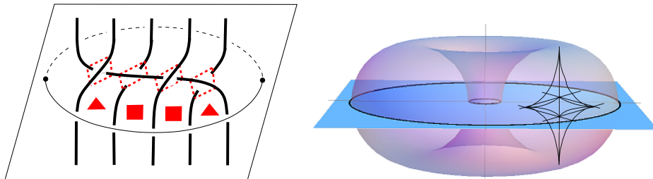
FIGURE 4. Left: Dividing projection plane into triangles and quadrilaterals. Right: Coning to ideal octahedra and tetrahedra, figure modified from [19].
