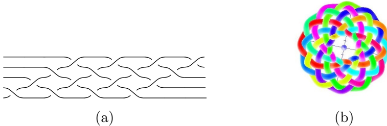
FIGURE 1. (a) W(5, 4) is the closure of this braid. (b) W(7, 12) figure modified from [23].
