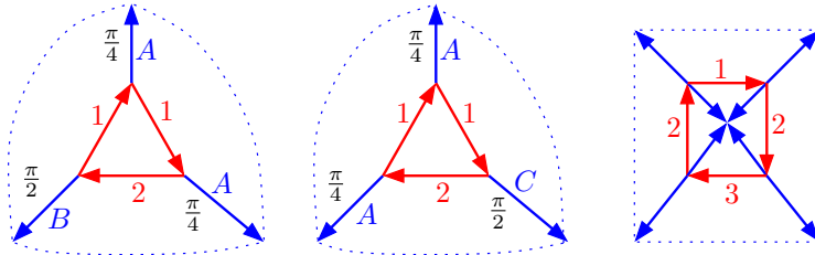
FIGURE 9. Edges are glued as shown in figure. From left to right, shown are tetrahedra T_1 , T_1' , and adjacent octahedron.
