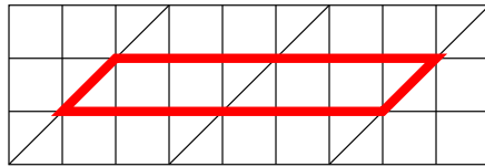
FIGURE 3. Polygonal decomposition of cusp corresponding to braid axis. A fundamental region consists of four triangles and 2(p-3) quads. The example shown here is p = 5 . The black diagonal is the preimage of a meridian.
