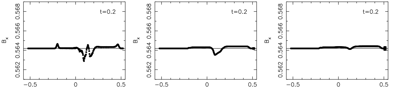
Figure 8. The parallel component of the magnetic field in the 2.5D shock tube problem using the usual dissipative terms (left), using the total magnetic energy (centre) and using the total magnetic and kinetic energies (right). Using the total magnetic energy in the dissipative terms means that jumps in the parallel field components are smoothed in addition to the jumps in transverse field. Using the total kinetic energy smooths jumps in the transverse (as well as parallel) velocity components, however this explicitly adds an undesirable shear component to the artificial viscosity term. Details of these formalisms are given in §5.
