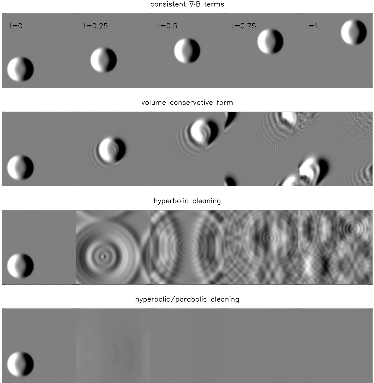
Figure 3. Results of the \nabla \cdot \mathbf{B} advection problem. An initially non-zero divergence is setup as a peak in the x -component of the magnetic field (leftmost figures), with a velocity field \mathbf{v}(x, y) = [1, 1] and periodic boundaries. The plots show renderings of \nabla \cdot \mathbf{B} in the range -1 < \nabla \cdot \mathbf{B} < 1 (from black to white) at various times throughout the simulation for various divergence cleaning procedures. The consistent treatment of \nabla \cdot \mathbf{B} terms (top row) is clearly seen to advect the divergence without change, which is an improvement over a “conservative” formulation of the MHD equations in which the divergence is smeared throughout the simulation volume (second row). With the use of hyperbolic cleaning in addition to the consistent \nabla \cdot \mathbf{B} terms, the divergence error is spread rapidly in a wavelike manner (third row), whilst with a mixed hyperbolic/parabolic cleaning (fourth row) this error is also quickly diffused away.
