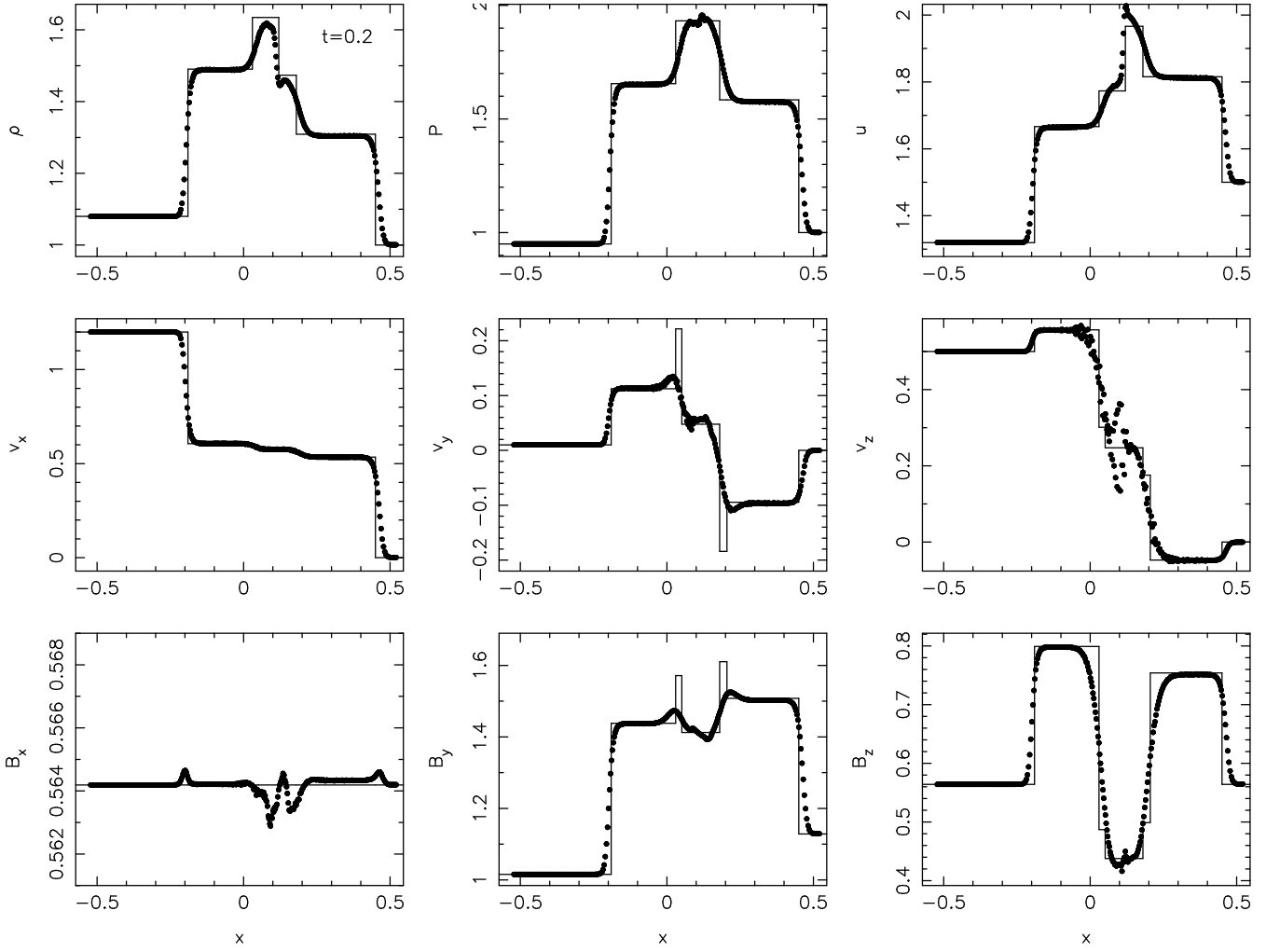
Figure 7. Results of the 2.5D shock tube test using 310 \times 4 particles and an initial smoothing length of h = 1.2(m/\rho)^{1/2} . In two dimensions at this value of smoothing length small oscillations in the transverse velocity components appear primarily as a result of the non-zero magnetic divergence. In this plot the usual artificial viscosity and resistivity terms have been applied uniformly (ie. not using switches). A small amount of artificial thermal conductivity has been applied using the switch.
