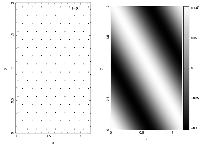
Figure 5. Circularly polarized Alfvén wave test. The left figure shows the particle setup in the lowest resolution simulation. On the right the vertical component of the magnetic field is plotted as a rendered image from the 32 \times 64 particle run at t = 5 , showing the propagation of the wave with respect to the domain and the particle setup.
