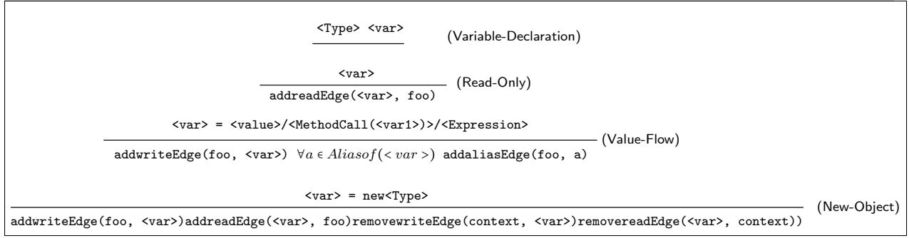
Fig. 3. Statement Rules.
