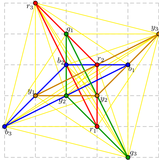
FIGURE 1. A \{3, 3, 3, 3\} -blocked point set.
