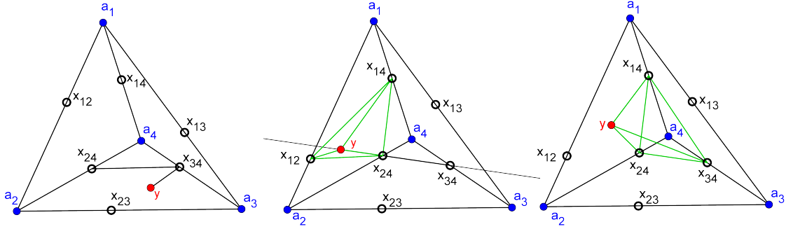
FIGURE 6. Diagrams of \{4, 3, 2, 2\} cases 1, 2, and 3.
