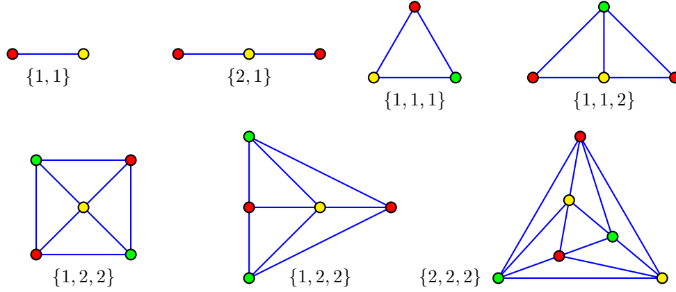
FIGURE 2. The 2-blocked and 3-blocked point sets.
