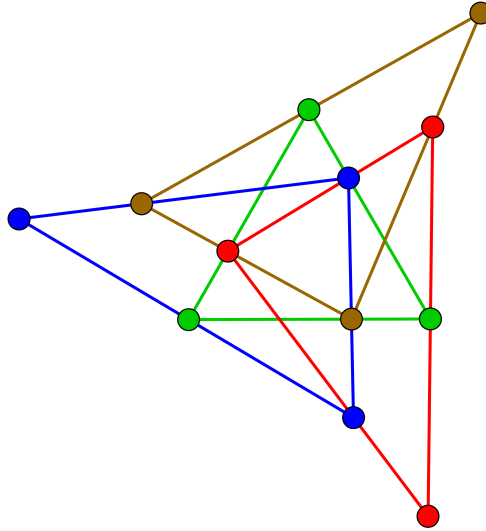
FIGURE 8. Another \{3, 3, 3, 3\} -blocked point set.
