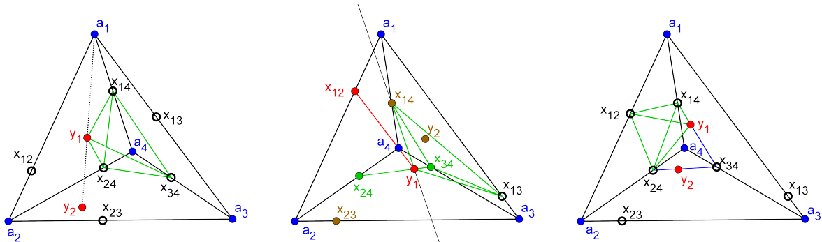
FIGURE 7. Diagrams of \{4, 3, 3, 2\} cases 1, 2, and 3.
