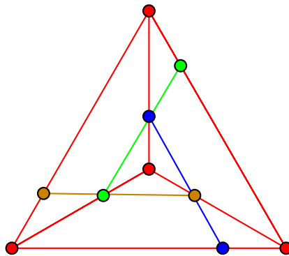
FIGURE 5. A \{4, 2, 2, 2\} -blocked point set.
