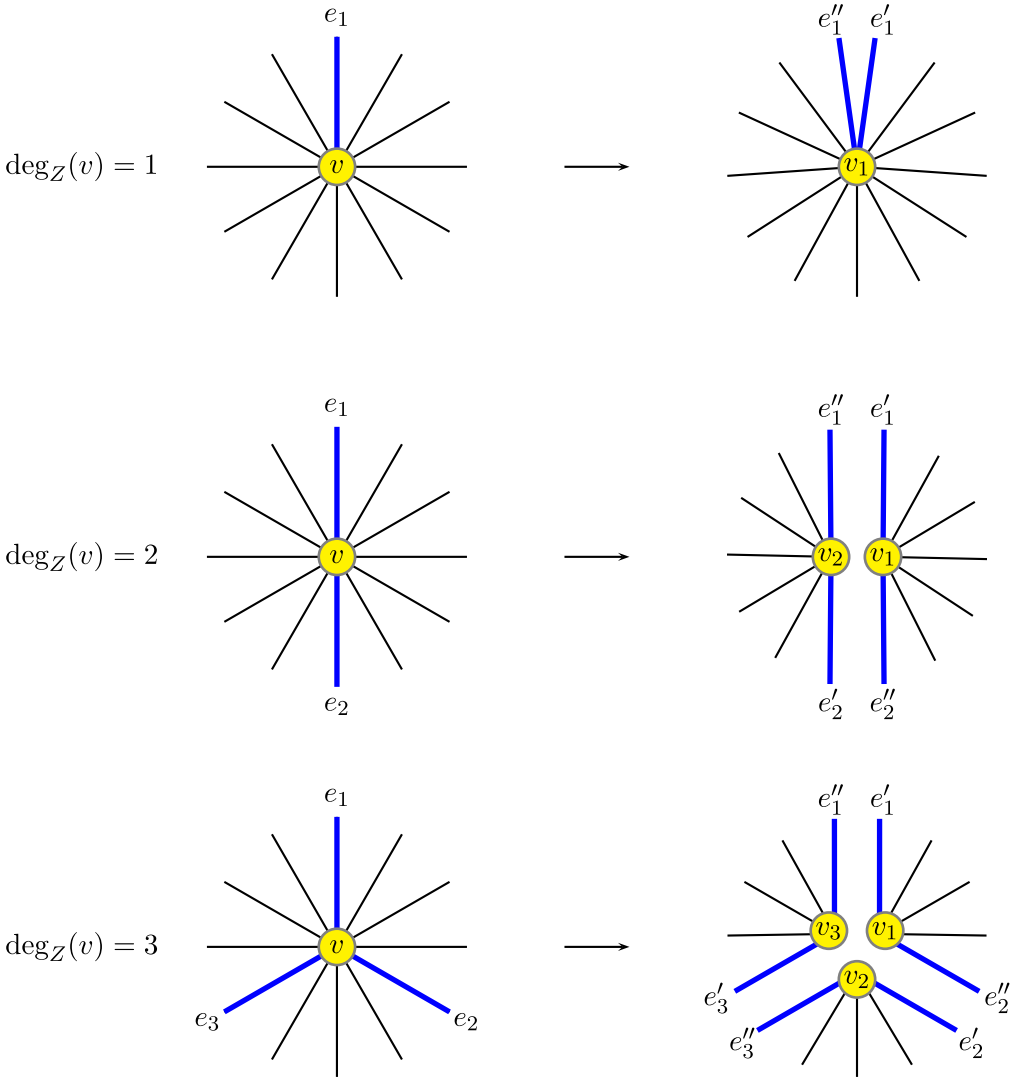
Fig. 3. Cutting the blue edges in Z at each vertex.
