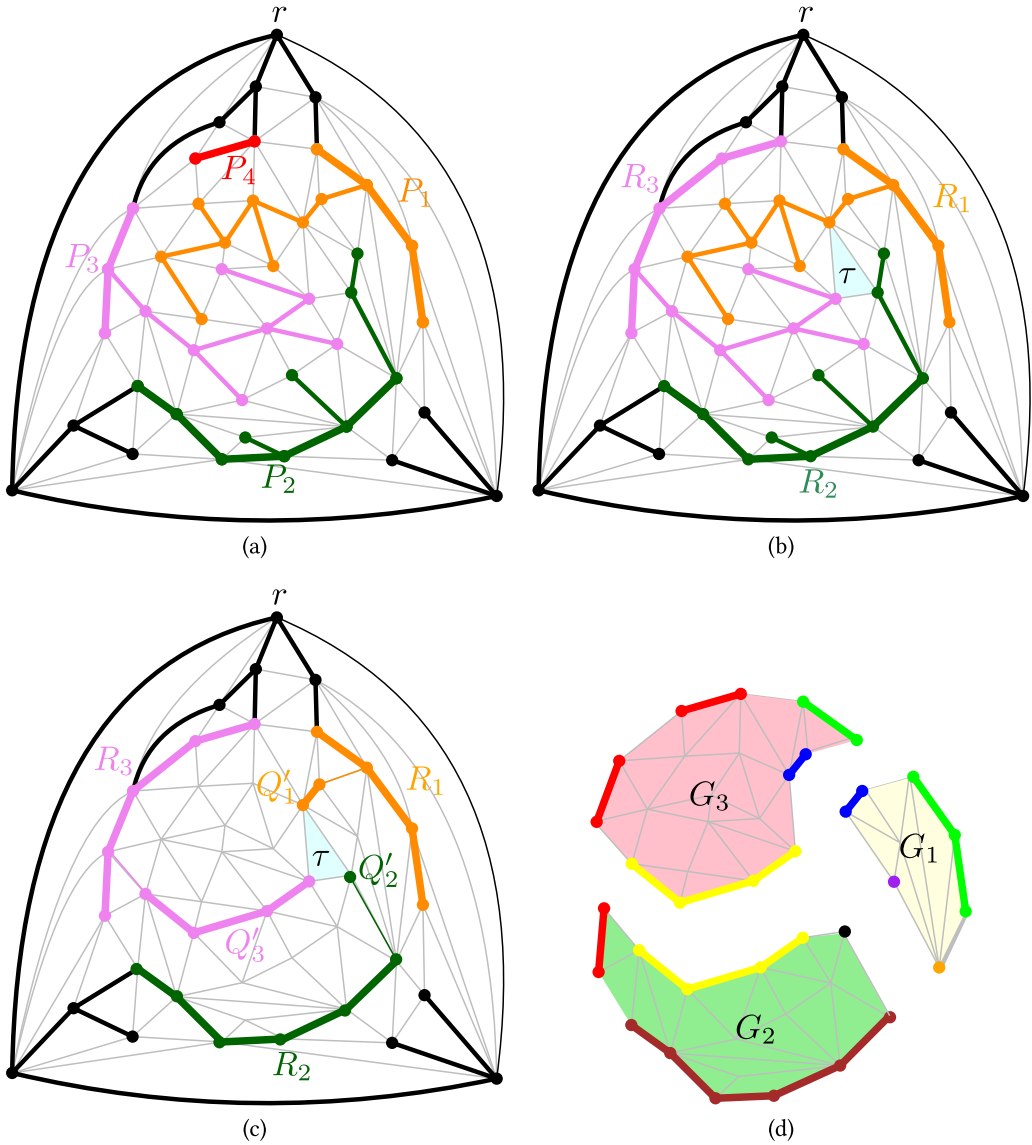
Fig. 2. The inductive proof of Lemma 13: (a) the spanning tree T and the paths P_1, \dots, P_4 ; (b) the paths R_1, R_2, R_3 , and the Sperner triangle \tau ; (c) the paths Q'_1, Q'_2 and Q'_3 ; (d) the near-triangulations G_1, G_2 , and G_3 , with the vertical paths of T on F_1, F_2 , and F_3 .
