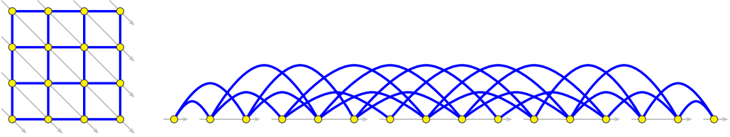
Fig. 1. 1-Queue layout of grid graph.
