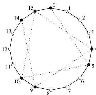
Fig. 2. A rhythm with k=7 onsets and timespan n=16 that is Winograd-deep and thus Erdős-deep. Distances ordered by multiplicity from 1 to 6 are 2, 7, 4, 1, 6, and 5. The dotted line shows how the rhythm is generated by multiples of m=5 .
